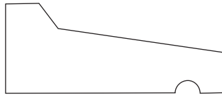
CM197 11/16 X 1-5/8 Drip Cap
