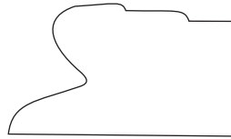
KCR615FJ 3/4 X 1-3/8 Stucco Mold
