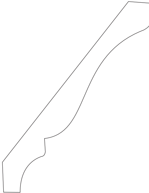
TO048 9/16 X 4-3/16 Crown
